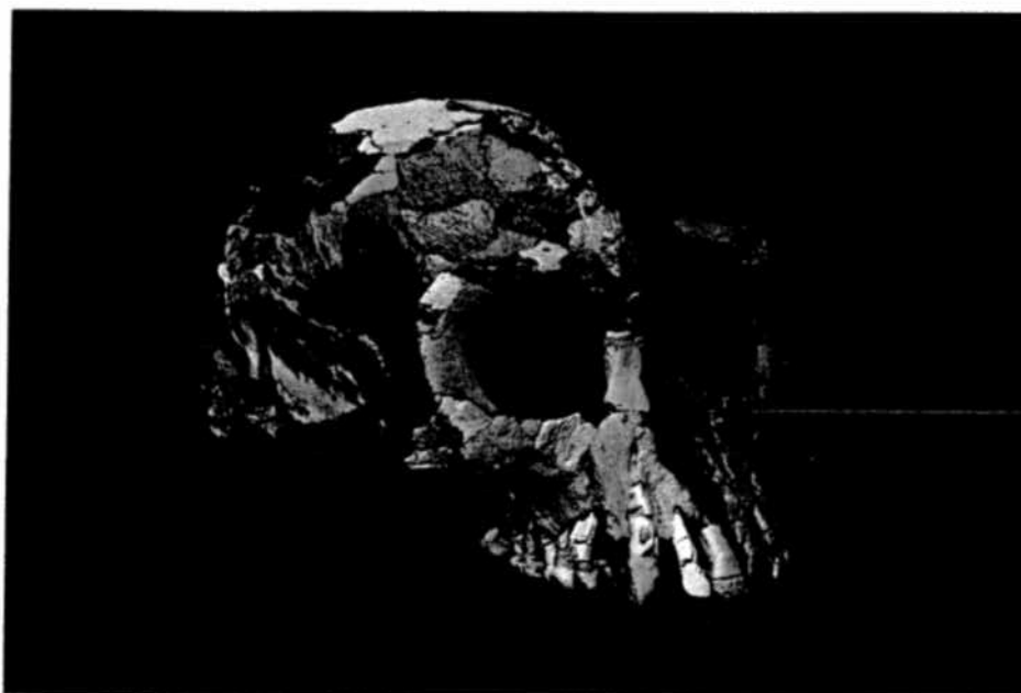
fossils, he pieced together 64 digital fragments. Checking his work against other ancient and modern primates, Suwa rebuilt a virtual skull and made a mirror image of part of the face to create its missing left side (brown section). He assigned colors to the rest of the pieces to differentiate them.
